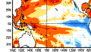
Jun–Jul–Aug 2024
